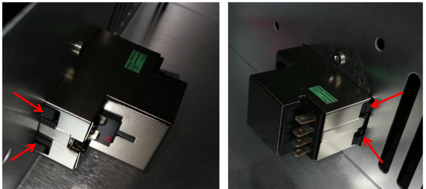
Figure 7 Power switch removal
