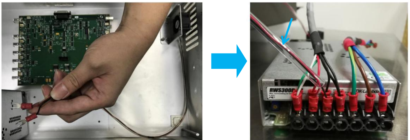
Figure 20 Ventilation Fan Power Cable Connection
