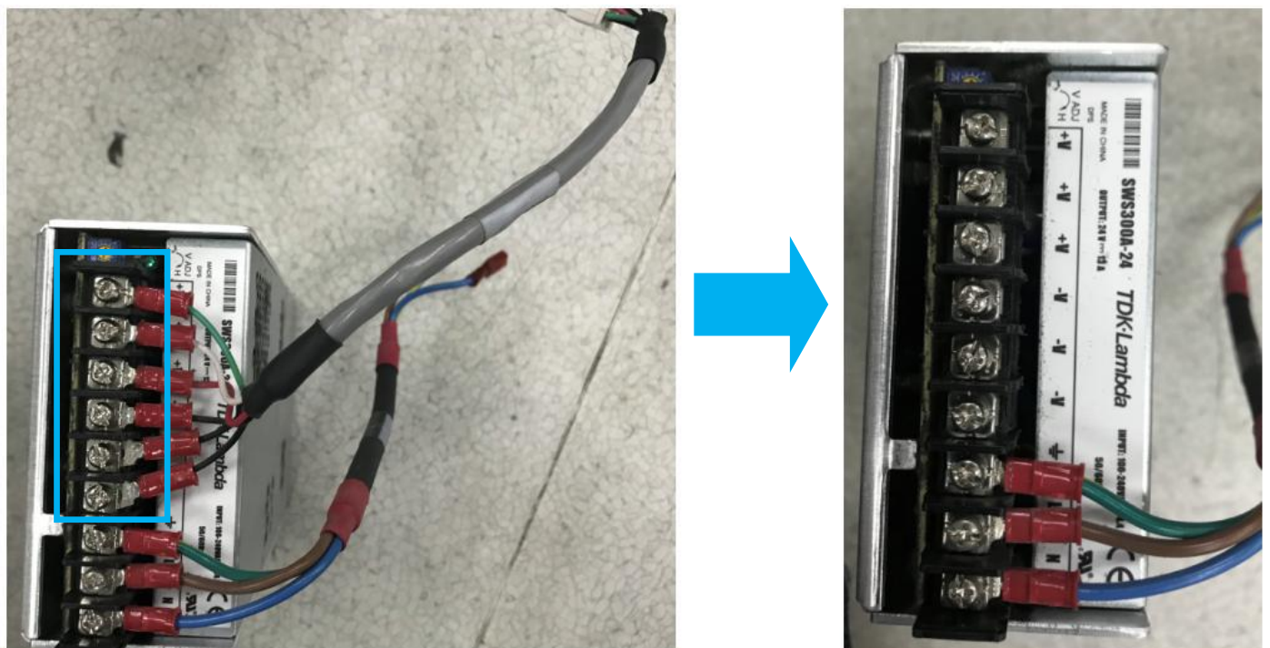
Figure 14 Trigger Board End Power Cable removal
