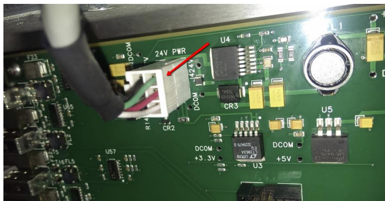
Figure 4 Trigger board power removal
