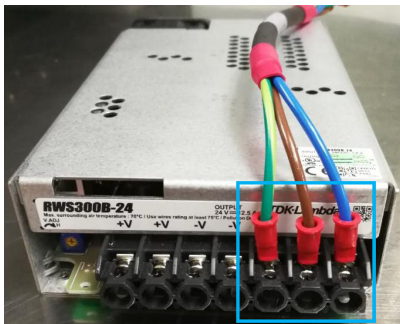
Figure 18 Power Switch Cable Connection
