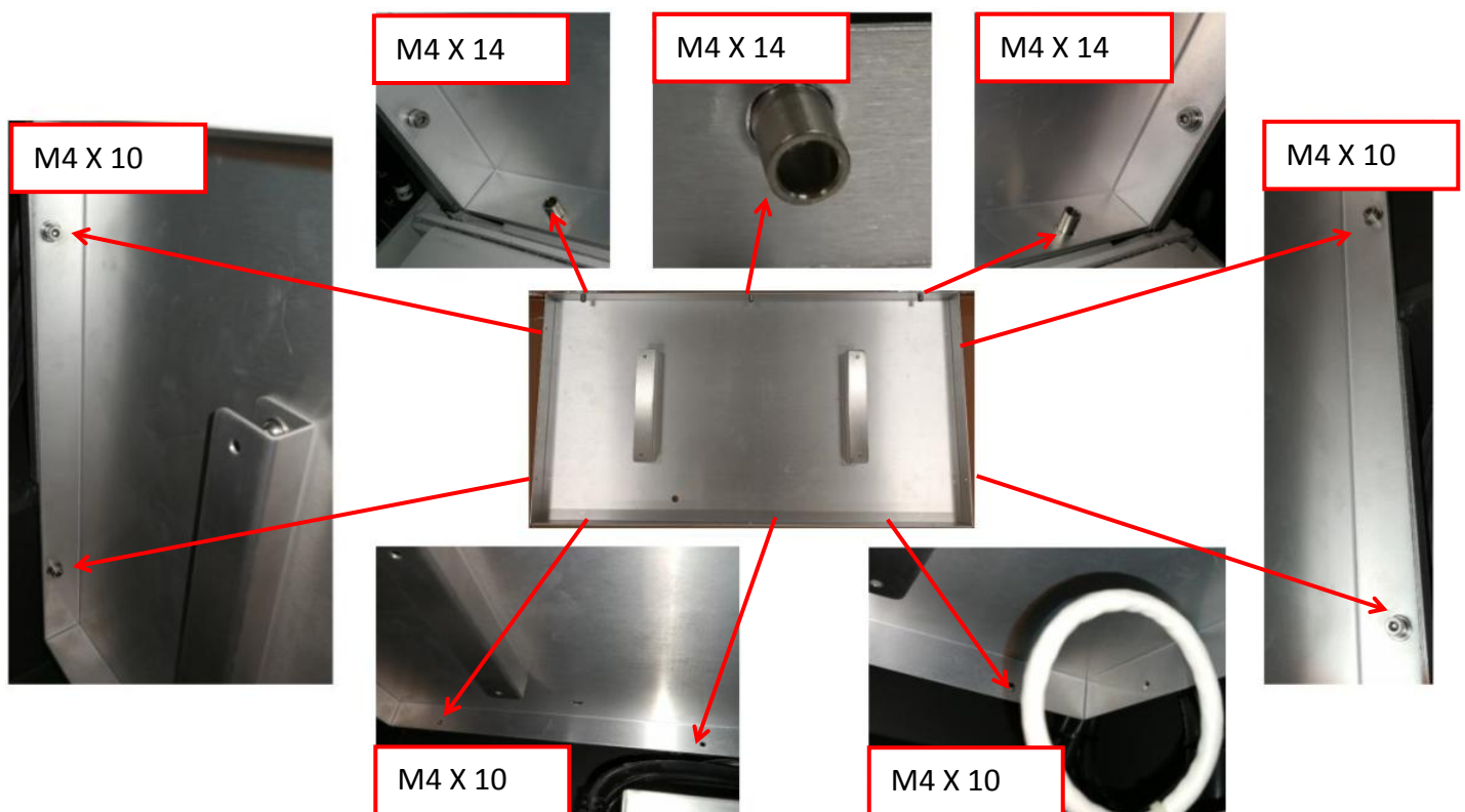
Figure 33 Trigger Board Tray Cover assembly
