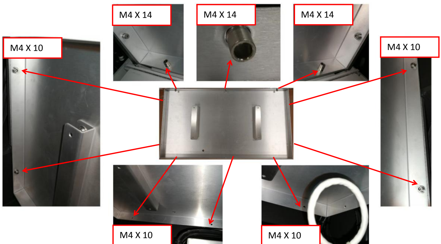
Figure 2 Trigger board Tray Cover removal
