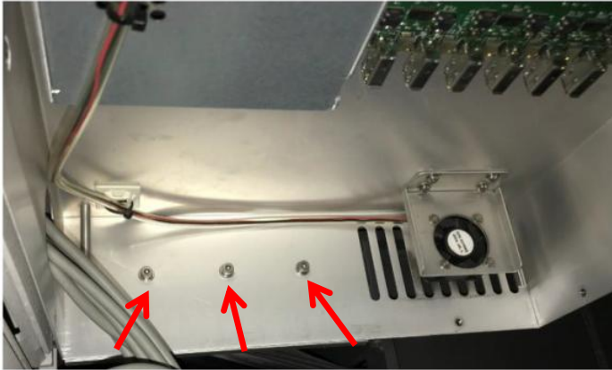
Figure 8 Trigger Board Tray removal
