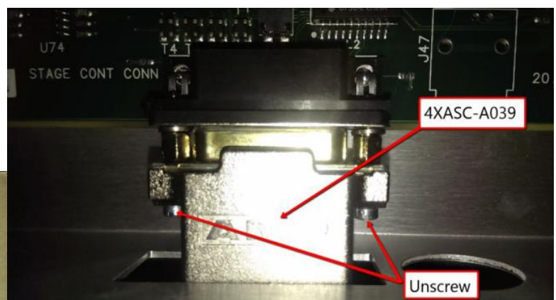
Figure 5 Connector removal
