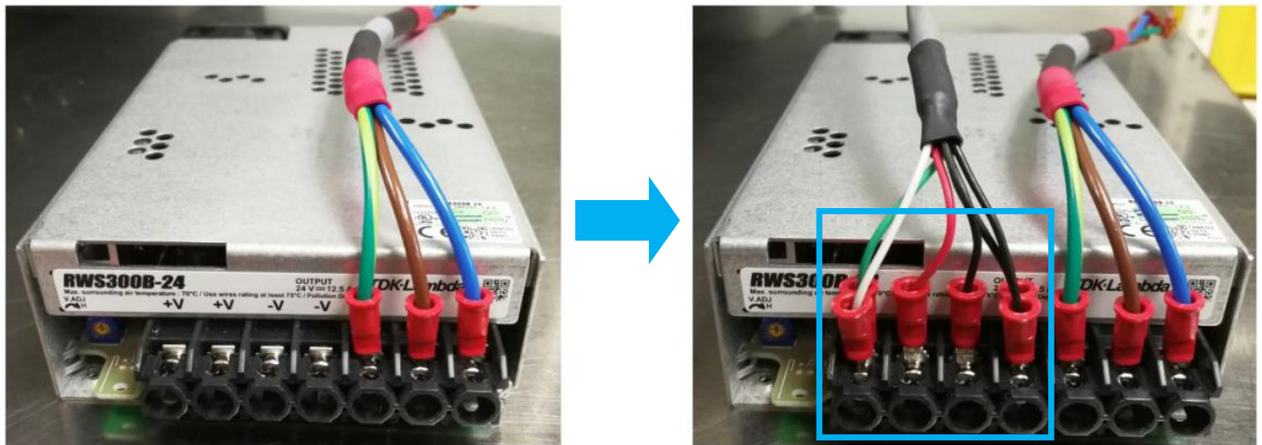
Figure 19 Trigger Board End Power Cable Connection
