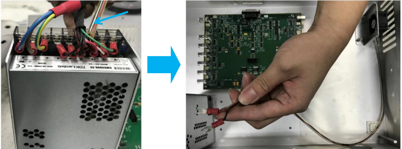
Figure 13 Ventilation Fan Power Cable Removal
